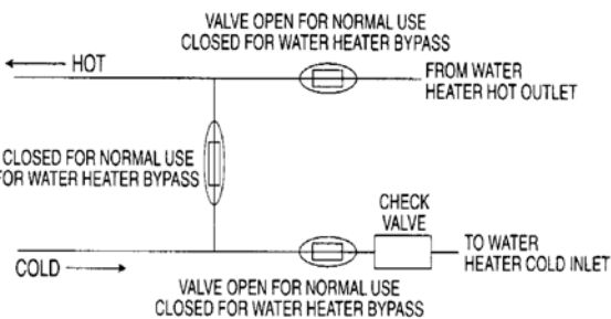
Water Heater Bypass Valve diagram
