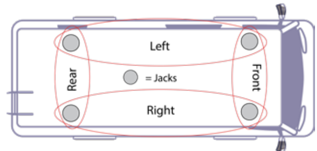
Hydraulic Leveling Diagram indicating jacks operate in pairs.
