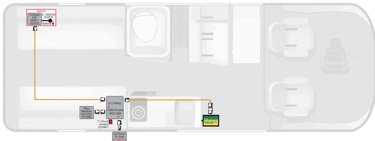
Wiring illustration (above) of a typical Firefly multiplex system; consisting of main touchscreen control panel, wireless room switches, and main electrical control board.
